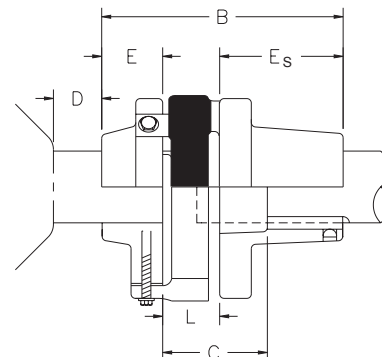
TYPE ES SINGLE SPACER COUPLING
