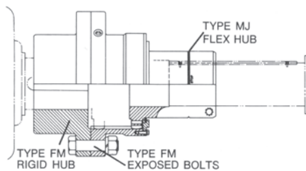
Type JMS Flex-Rigid
