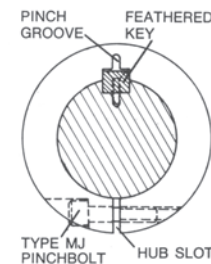
Section View of Type MJ Slide Hub on a Shaft
