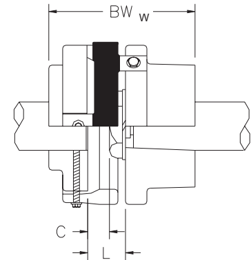
WIDE MOUNT
