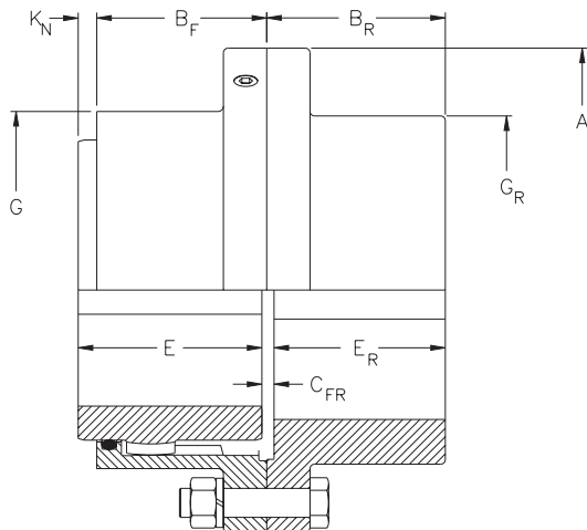
Flex-Rigid Coupling Data
