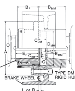
Type DRW
