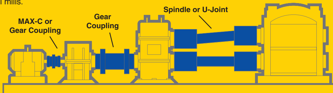
Typical Rolling Mill Main Drive with Complete Coupling/Spindle Selection
