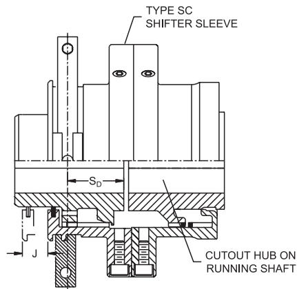
Type FCC Cutout Coupling
