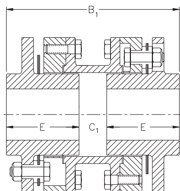
STANDARD HUBS STANDARD HUBS
