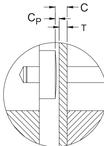
ALTERNATE SHAFT END CONFIGURATION ARRANGEMENT 'A' (ALTERNATE)
