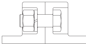
SHROUDED BOLTS
