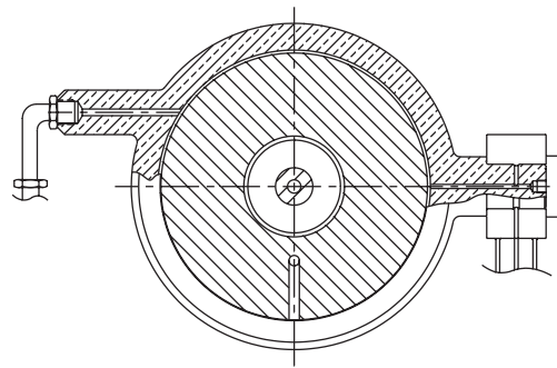
SECTION "B"~"B" LUBE RING
