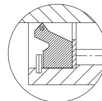
Lip Seal
