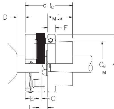
CLOSE MOUNT
