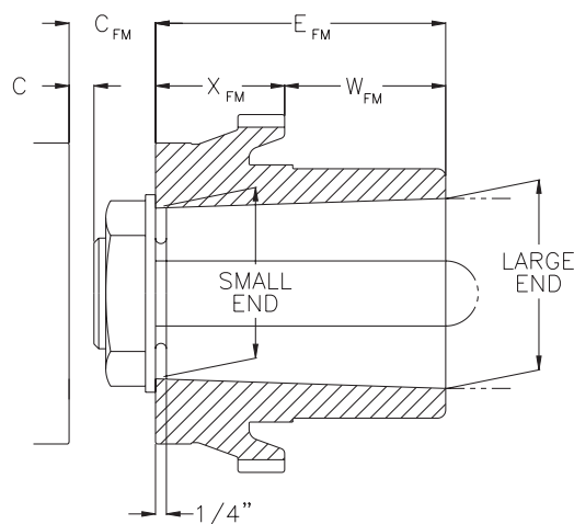
MILL MOTOR COMPOSITE HUB FINISH BORED
