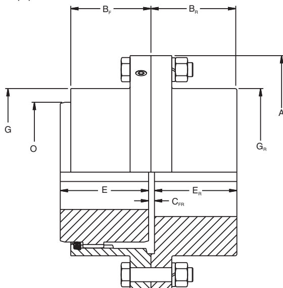
Coupling Type SB (Shrouded Bolts) Part Numbers
